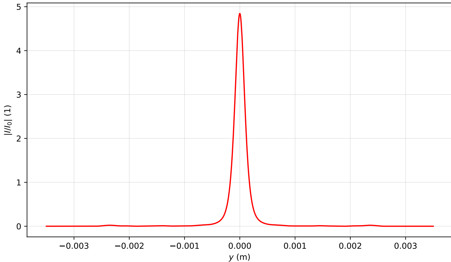
Intensity profile I(x=0, y, z=3.582)/I_0 , \text{Pin}=2.5\text{Pcr} , artificial time
